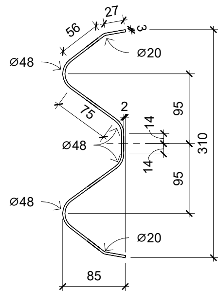
SCALE 1:5
